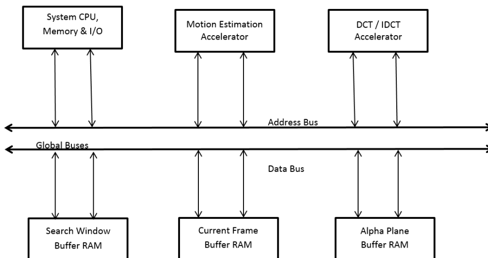
Fig 9: Video Encoder System Architecture
