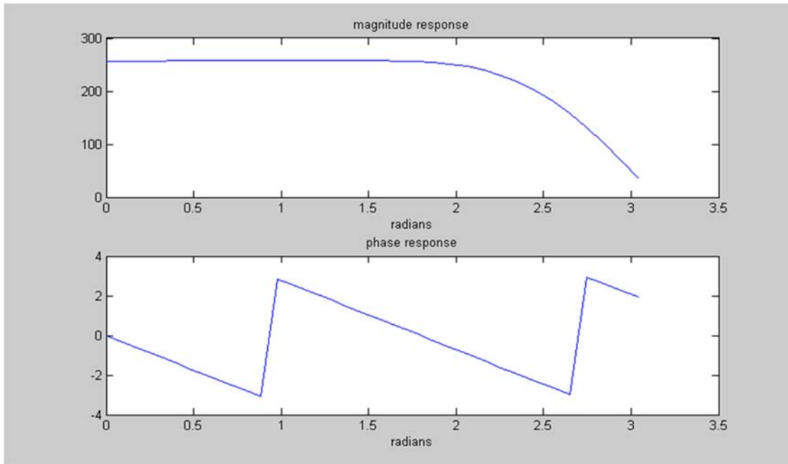
Fig 8: FIR Filter Response
