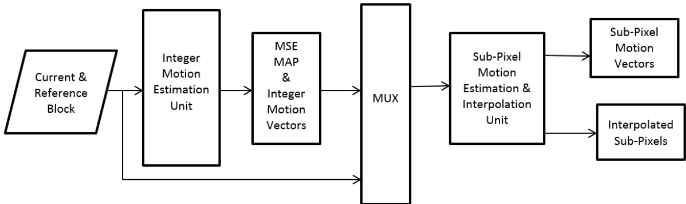
Fig 10: The Sub-Pixel Estimator
