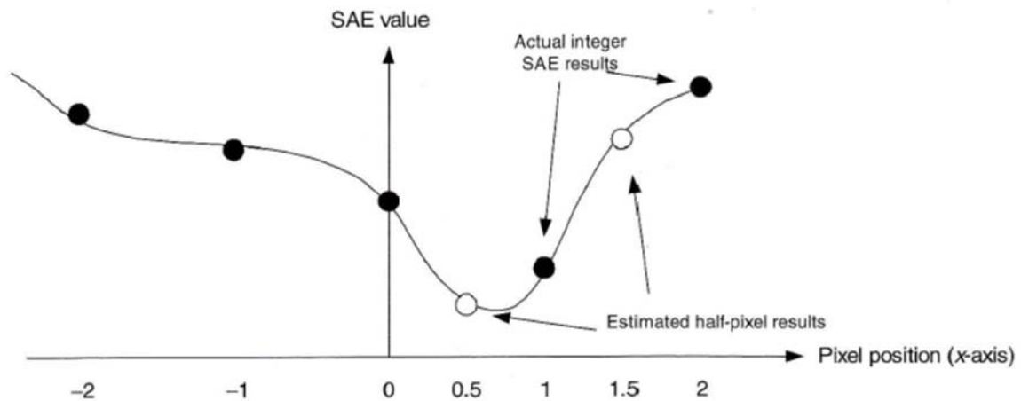
Fig 6: Estimating half-pixel positions from and Curve Fitting
