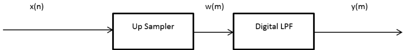
Fig 5: Interpolation Process
