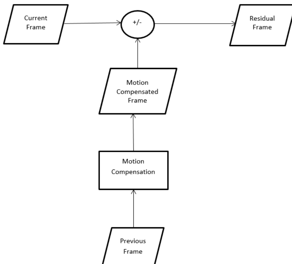
Fig 2: The Motion Compensator
