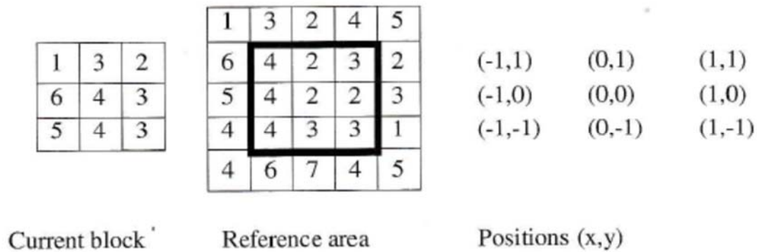
Fig 3: Block Matching Process and MSE positions
