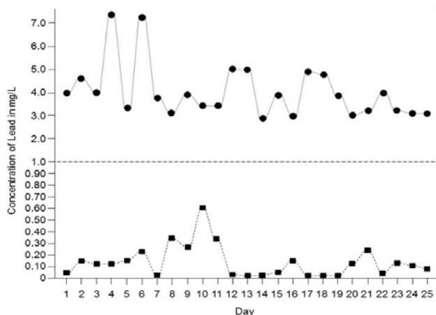
Fig 1: 25-day trend analysis of influent (top) and effluent (bottom) for lead concentrations in mg/L.
