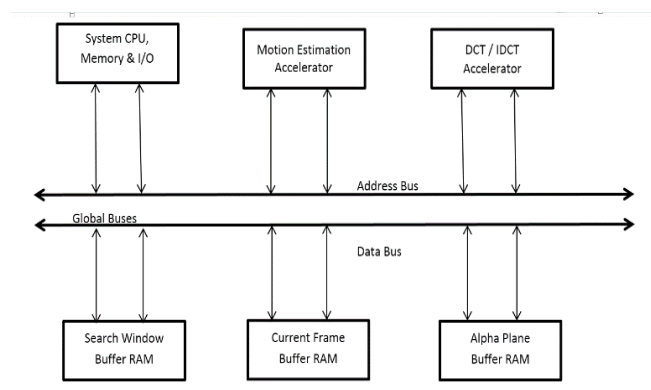
Fig 9: Video Encoder System Architecture
