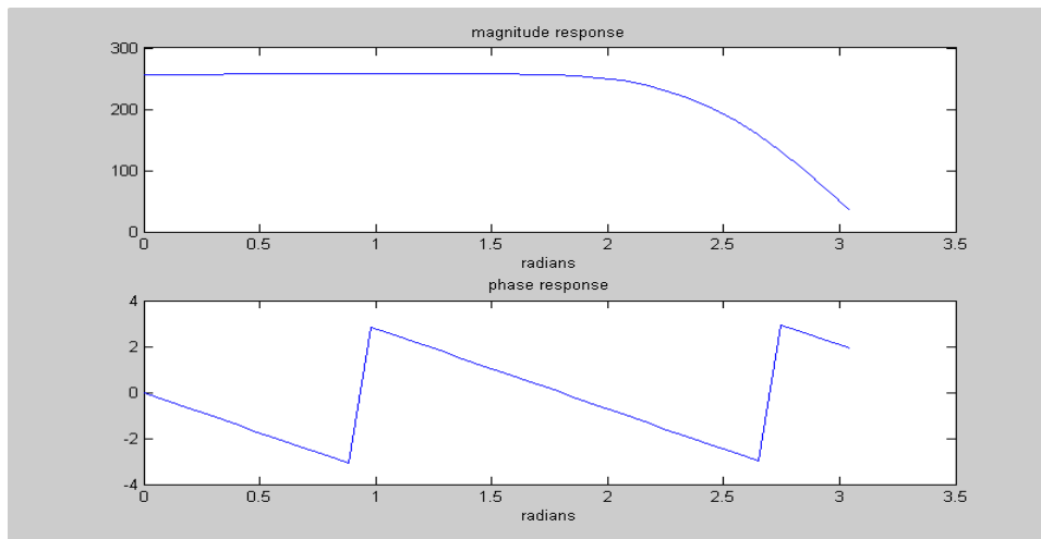
Fig 8: FIR Filter Response
