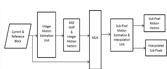
Fig 10: The Sub-Pixel Estimator
